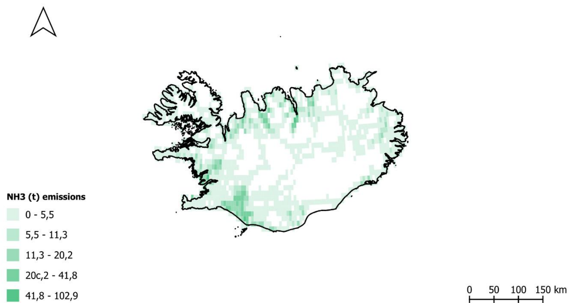
Figure 8.4: Emissions of NH 3 [t] in 2023.
