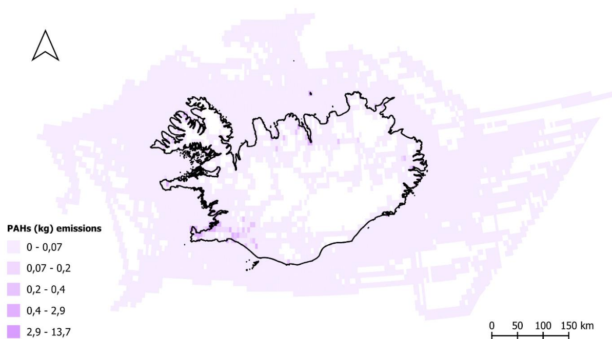
Figure 8.13: Emissions of PAHs [kg] in 2023.
