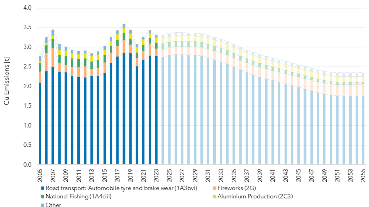
Figure 9.19 Cu emissions by main sources. Historical data and projections, 2005-2055.
