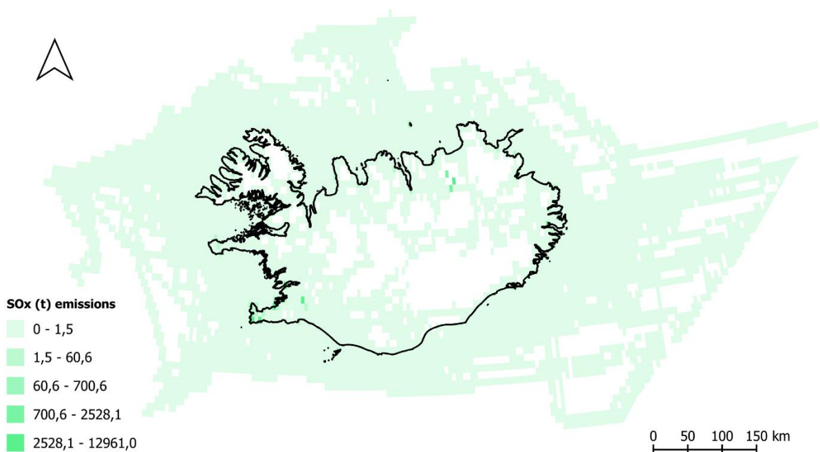
Figure 8.3: Emissions of SO x [t] in 2023.
