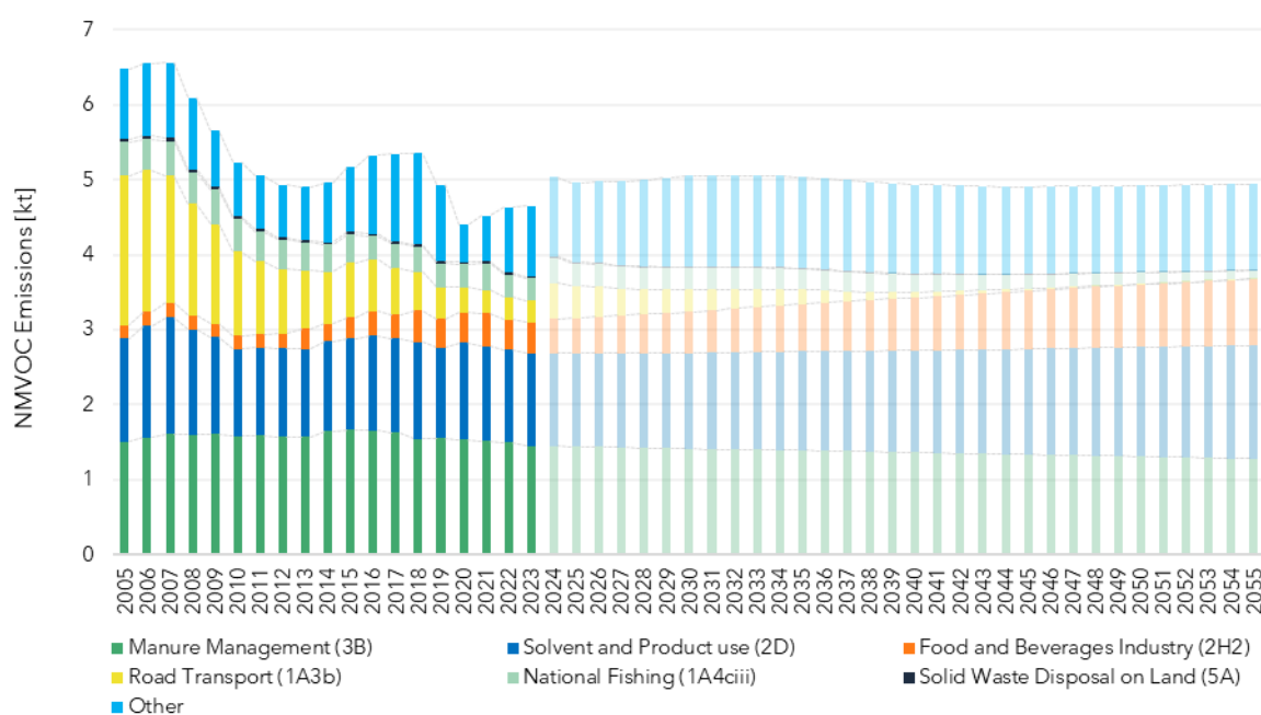
Figure 9.2 NMVOC emissions by main sources. Historical data and projections, 2005-2055.
