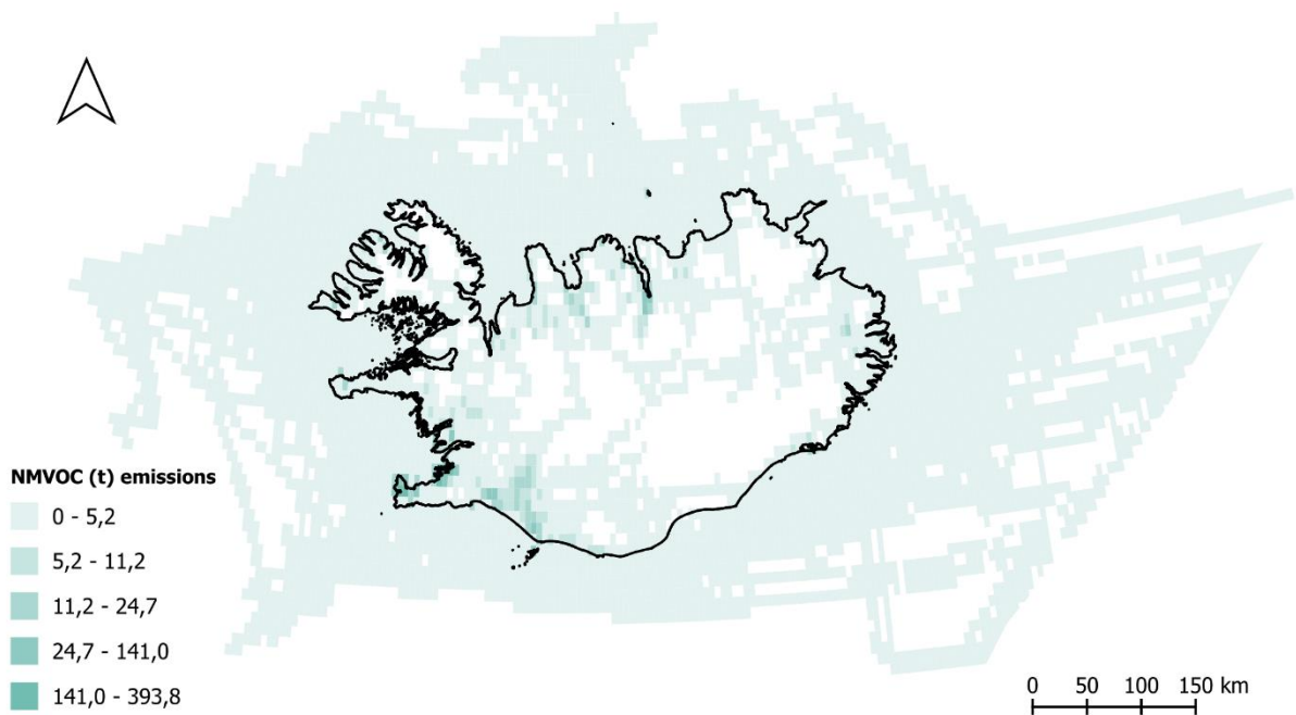
Figure 8.2: Emissions of NMVOC [t] in 2023.
