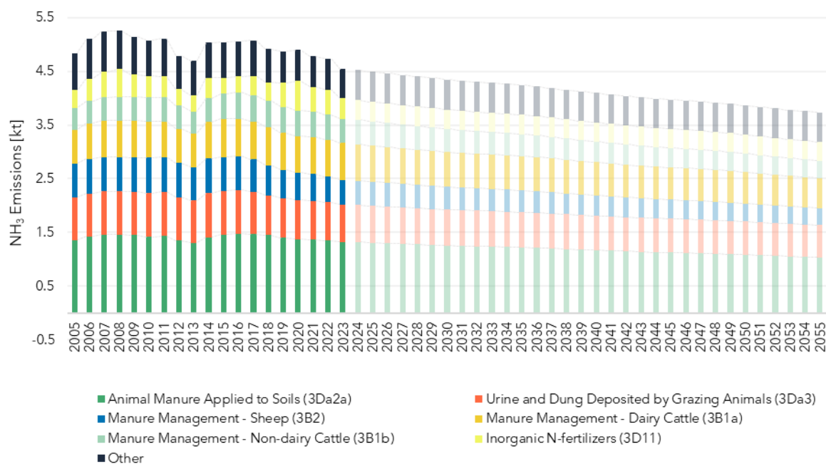
Figure 9.4 NH 3 emissions by main sources. Historical data and projections, 2005-2055.
