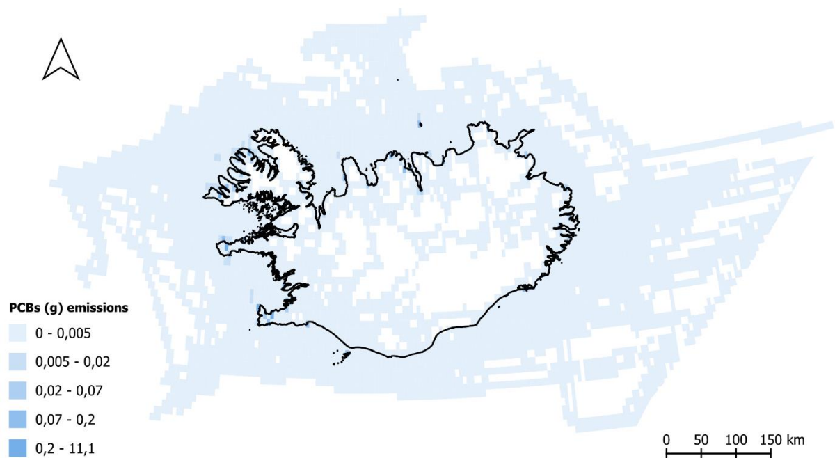
Figure 8.15: Emissions of PCBs [g] in 2023.
