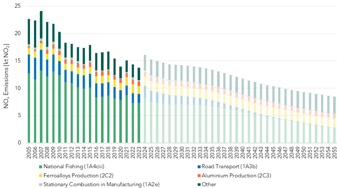
Figure 9.1 NO x emissions by main sources. Historical data and projections, 2005-2055.
