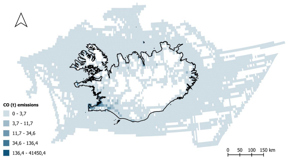
Figure 8.8: Emissions of CO [t] in 2023.
