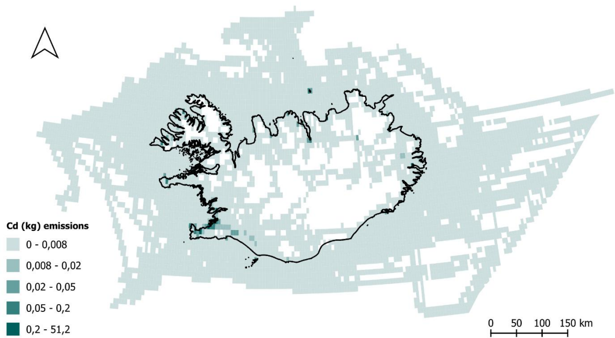
Figure 8.10: Emissions of Cd [kg] in 2023.
