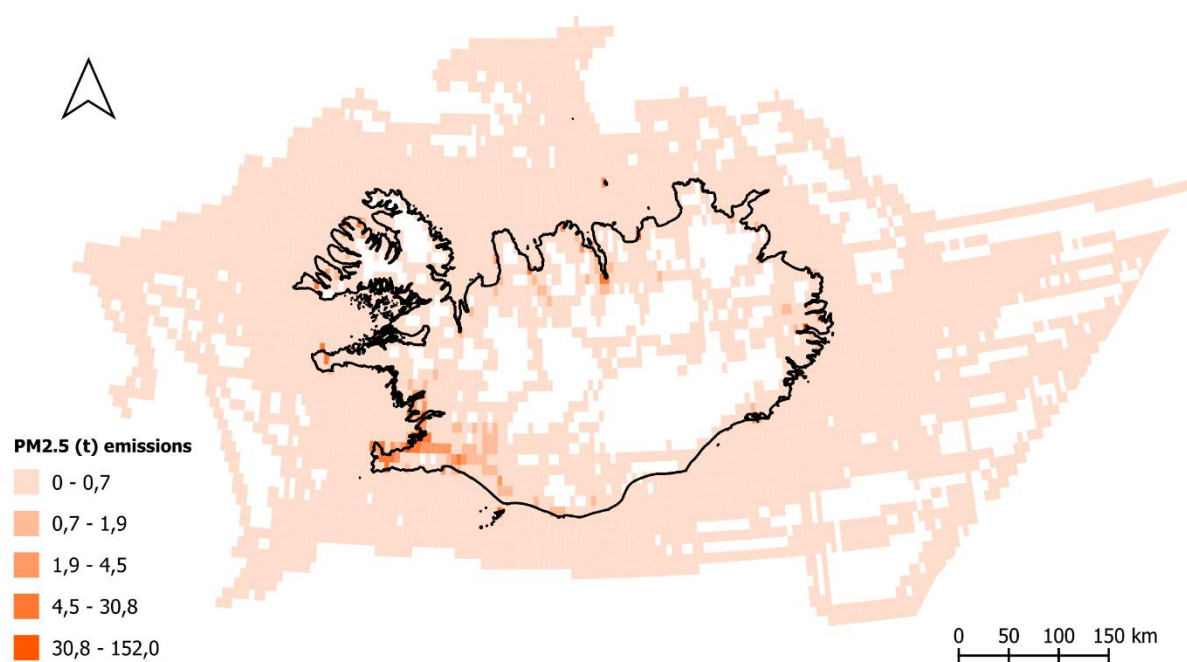
Figure 8.5: Emissions of PM 2.5 [t] in 2023.
