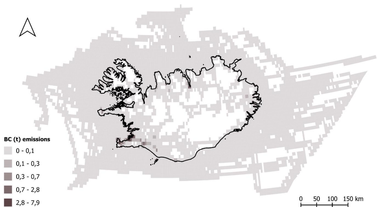
Figure 8.7: Emissions of BC [t] in 2023.
