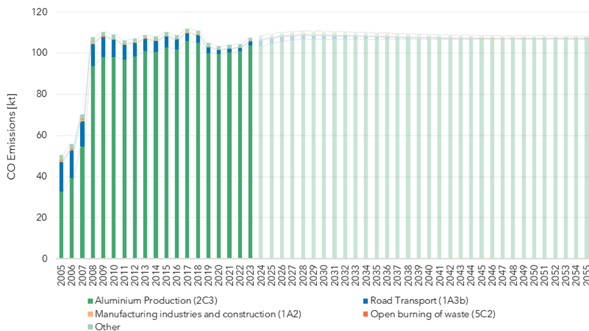
Figure 9.9 CO emissions by main sources. Historical data and projections, 2005-2055.
