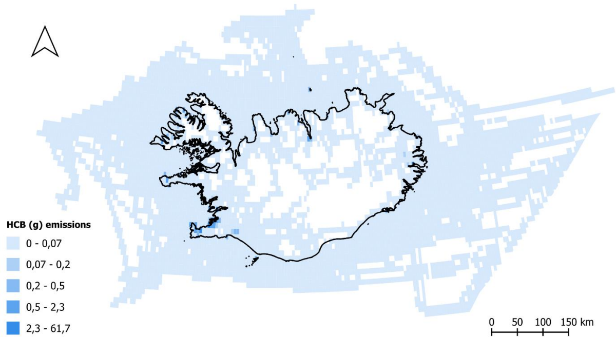
Figure 8.14: Emissions of HCB [g] in 2023.
