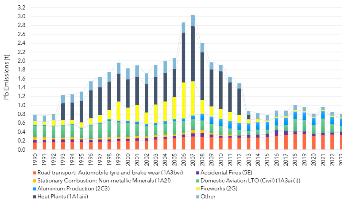
Figure 2.9 Pb emissions by sector, since 1990.
