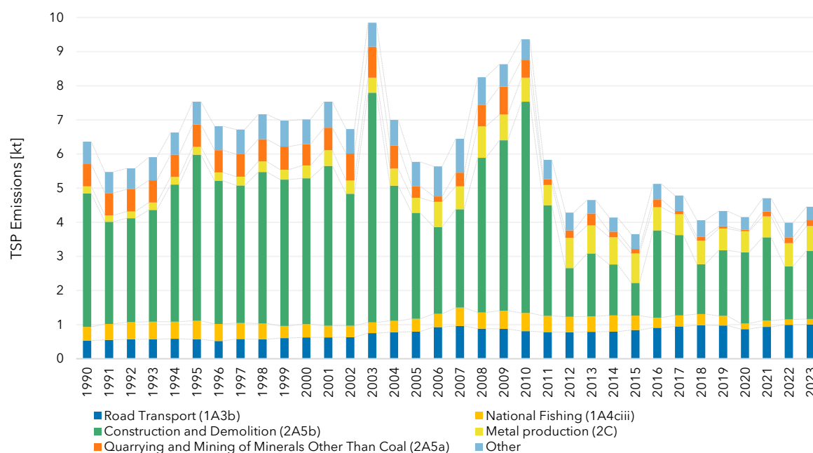
Figure 2.2 TSP emissions by sector, since 1990.
