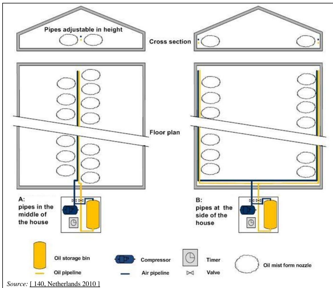
Figure 4.68: Schematic view of an oil spraying system
