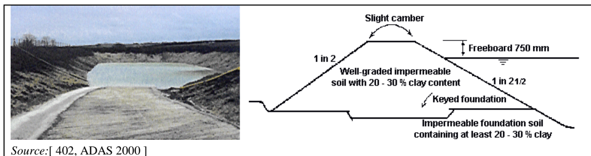
Figure 2.29: Example of earth-banked slurry store, and design features
